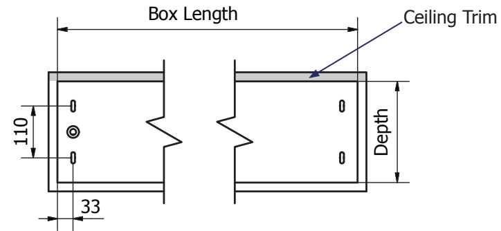
4 off Captive Nut Positions Ø5/16 Whitworth 2 at either end
